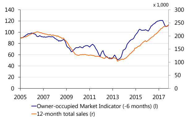
Chart 6: Confidence
